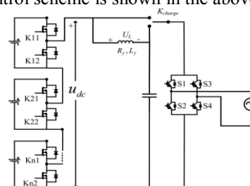
Fig 9. Charging circuit of cell with ac source
